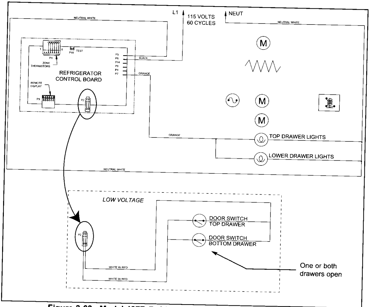
Figure 3-63. Model 427R Refrigerator Lighting System Signal Trace
