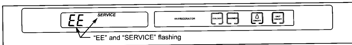
Figure 3-75. 427R Refrigerator Compartment Thermistor Fault, "EE" & "SERVICE" Flashing (Prior to Serial #1728753, "EE" and the Drawer Location Annunciators Will Flash)
