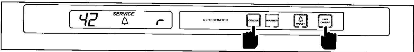
Figure 3-79. Initiating Diagnostic Mode, Press COLDER Key and UNIT ON/OFF key. First Reading is Refrigerator Compartment Temperature, Indicated by "r" (Prior to Serial #1728753, press UNIT ON/OFF Key Now to Identify Thermistor Location)
