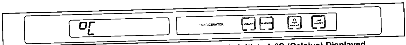
Figure 3-68. Initiating Temperature Units Selection Mode, Press and Hold THE Bell ON/OFF Key and Unit ON/OFF Key for 5 Seconds (Prior to Serial #1728753, Press and Hold THE "ALARM" Key and Unit ON/OFF Key for 5 Seconds)
