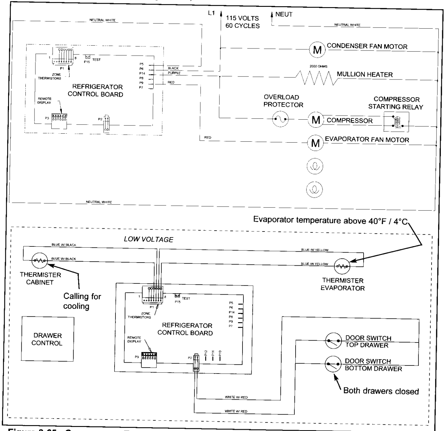
Figure 3-65. Compressor, Evap Fan, Mullion Heater & Condenser Fan Signal Trace, Refrigerator Section Calling for Cooling w/ Evaporator temperatures above 40°F / 4°C
