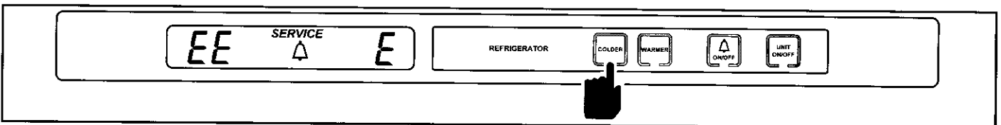
Figure 3-80. If "EE" is Displayed, Thermistor in that Location is Faulty (Prior to Serial #1728753, press UNIT ON/OFF Key Now to Identify Thermistor Location)
