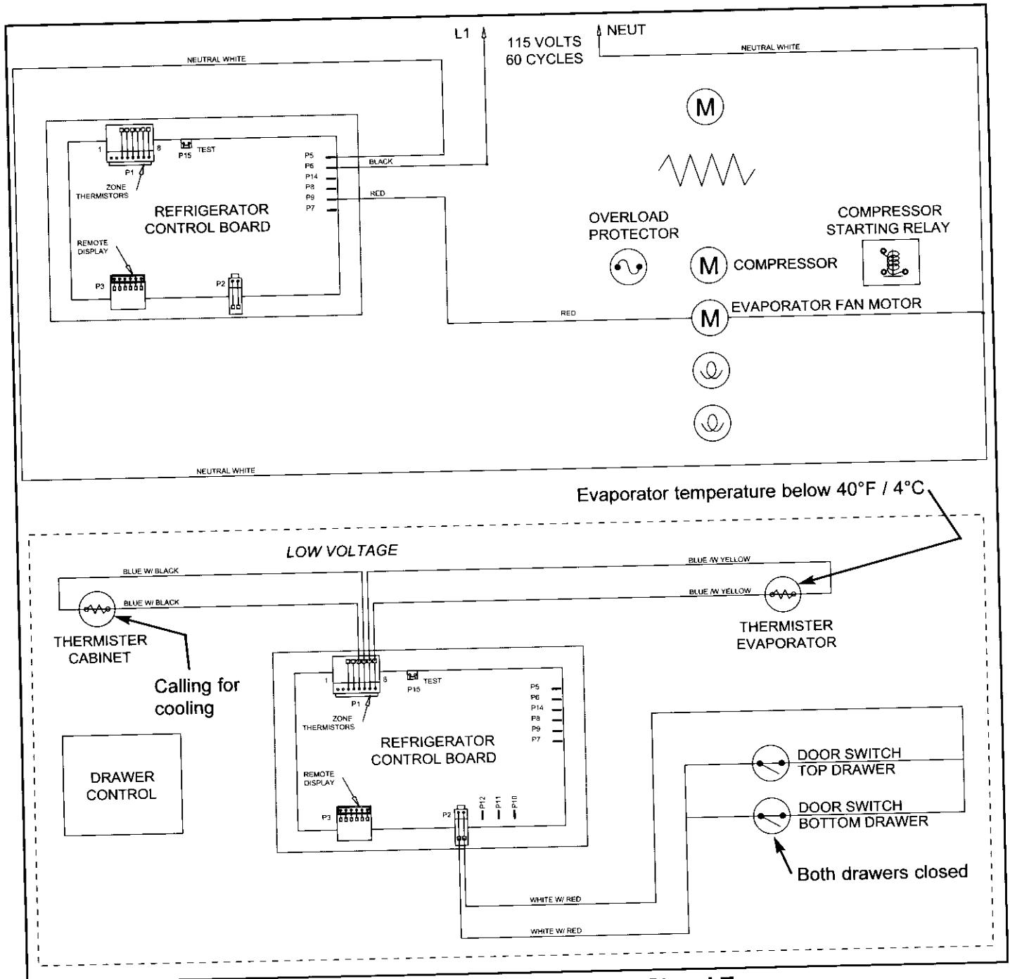
Figure 3-64. Evaporator Fan Power Signal Trace
