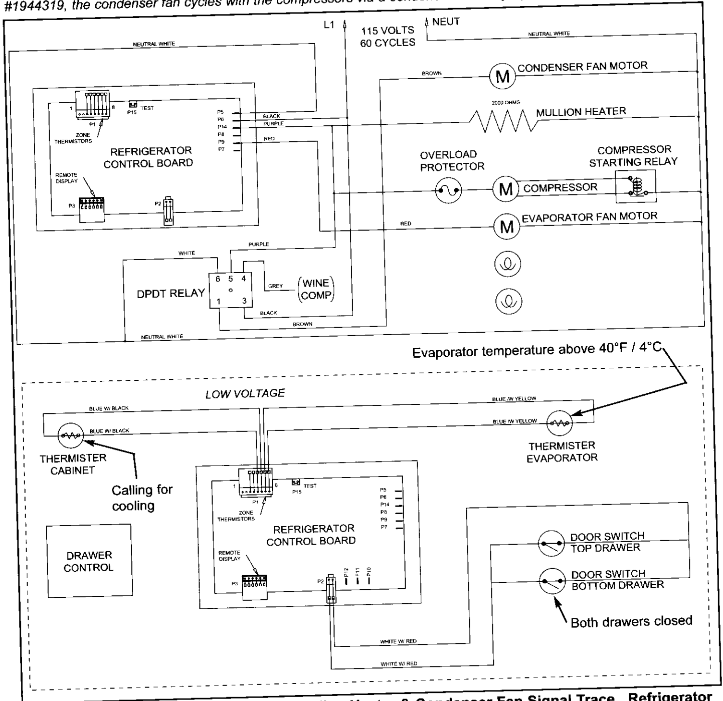
Figure 3-66. Compressor, Evap Fan, Mullion Heater & Condenser Fan Signal Trace, Refrigerator Section Calling for Cooling w/ Evaporator temperatures above 40°F / 4°C
