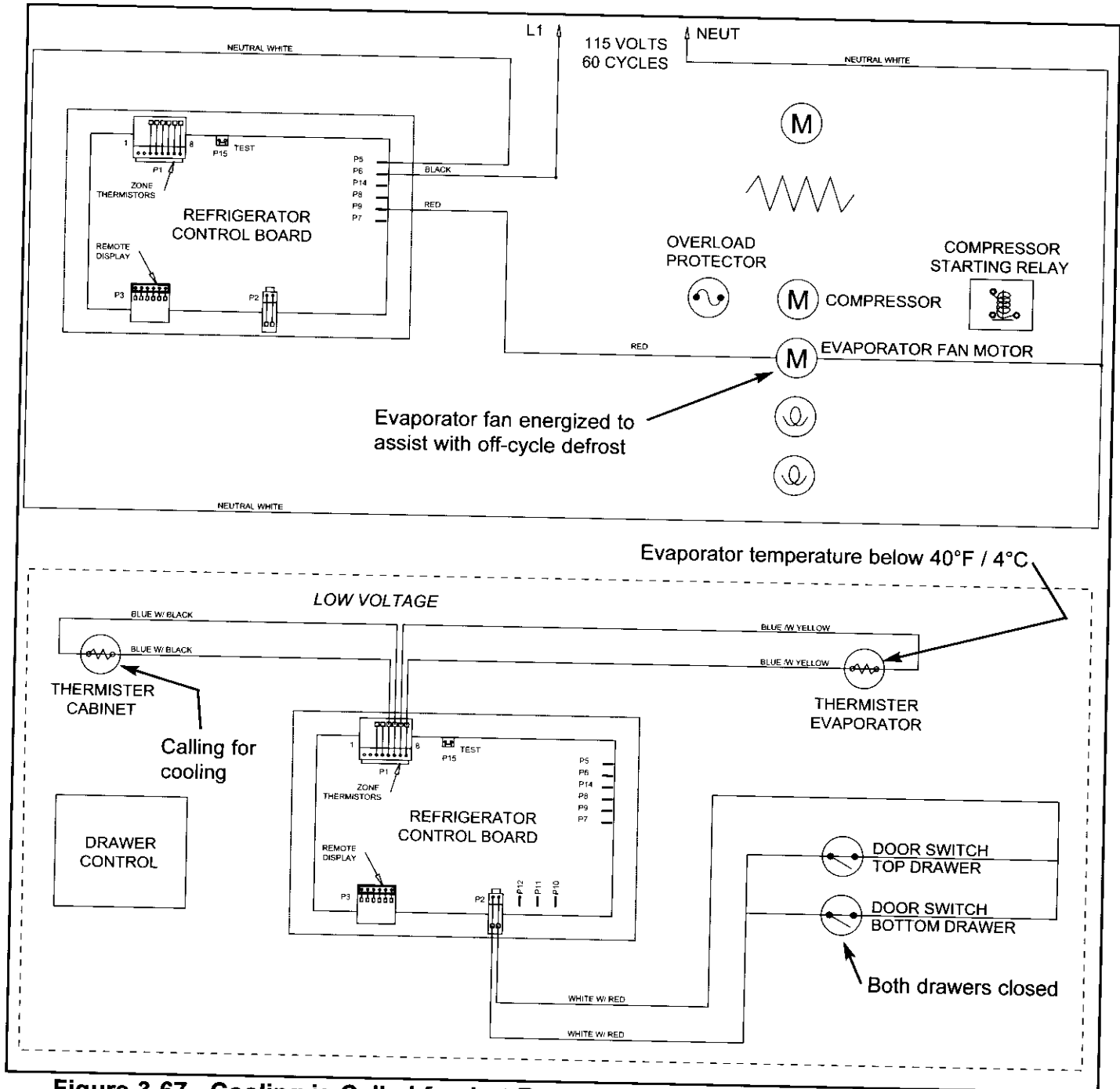
Figure 3-67. Cooling is Called for, but Evaporator Temperature is Below 40°F / 4°C, Compressor Waits for Evaporator to Fully Defrost
