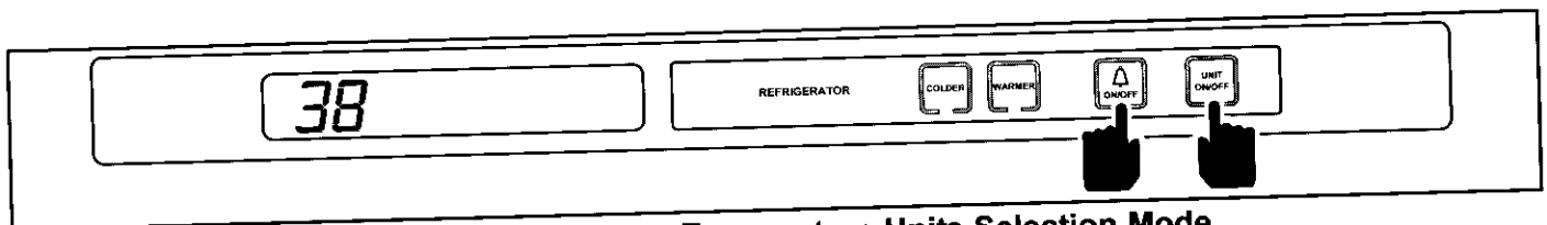
Figure 3-68. Initiating Temperature Units Selection Mode, Press and Hold THE Bell ON/OFF Key and Unit ON/OFF Key for 5 Seconds (Prior to Serial #1728753, Press and Hold THE "ALARM" Key and Unit ON/OFF Key for 5 Seconds)
